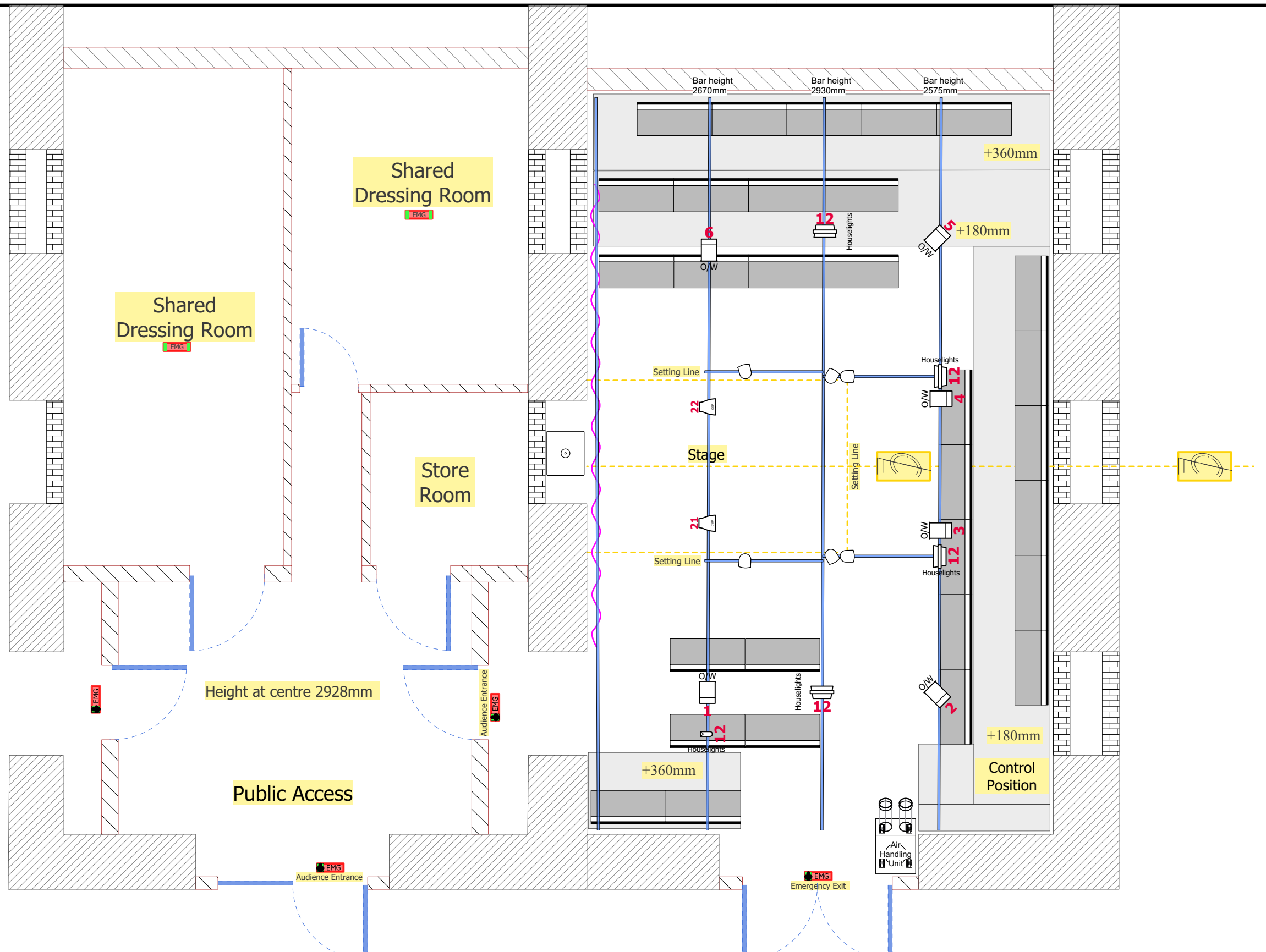
1 Pleasance Bunker One - Website - A3 Scale: 1:50
