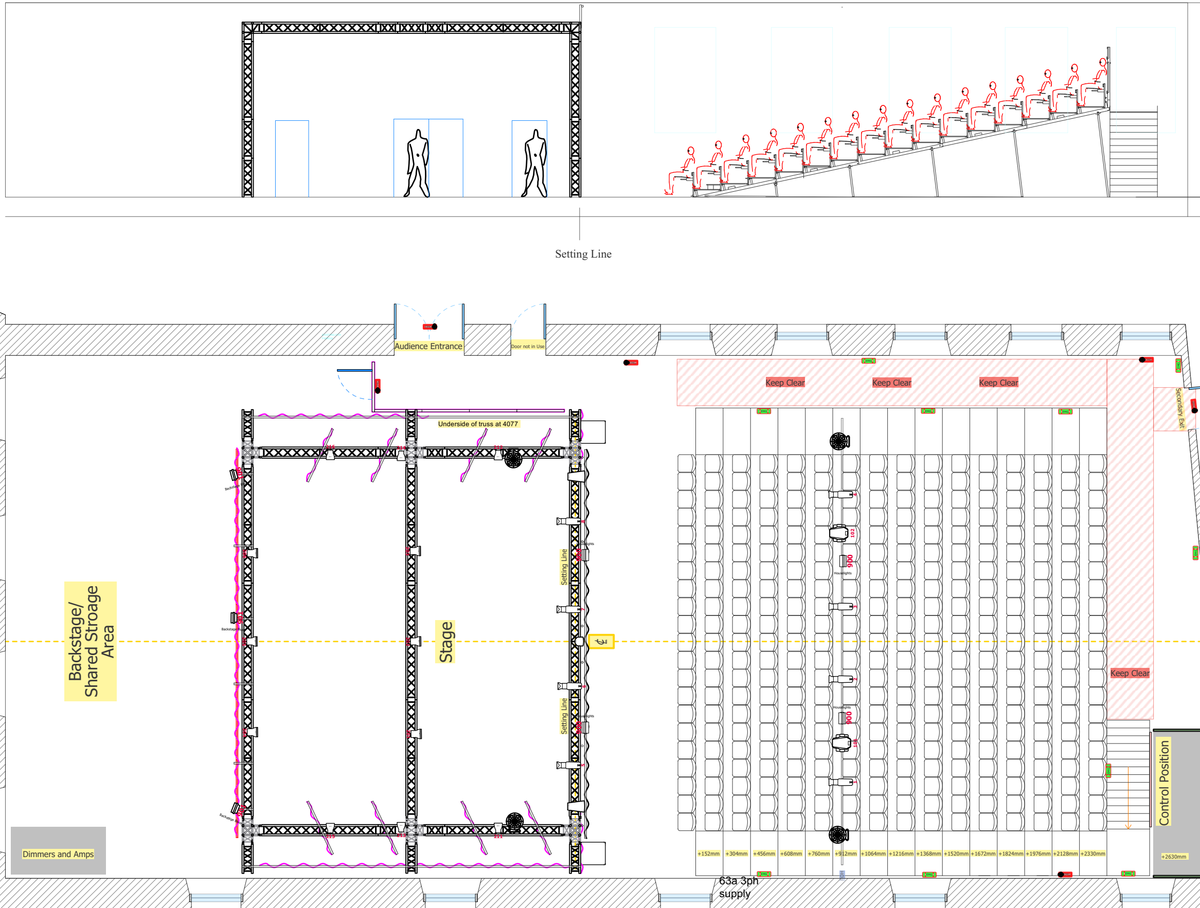
2 Pleasance Beyond -Website View A3 Scale: 1:100
