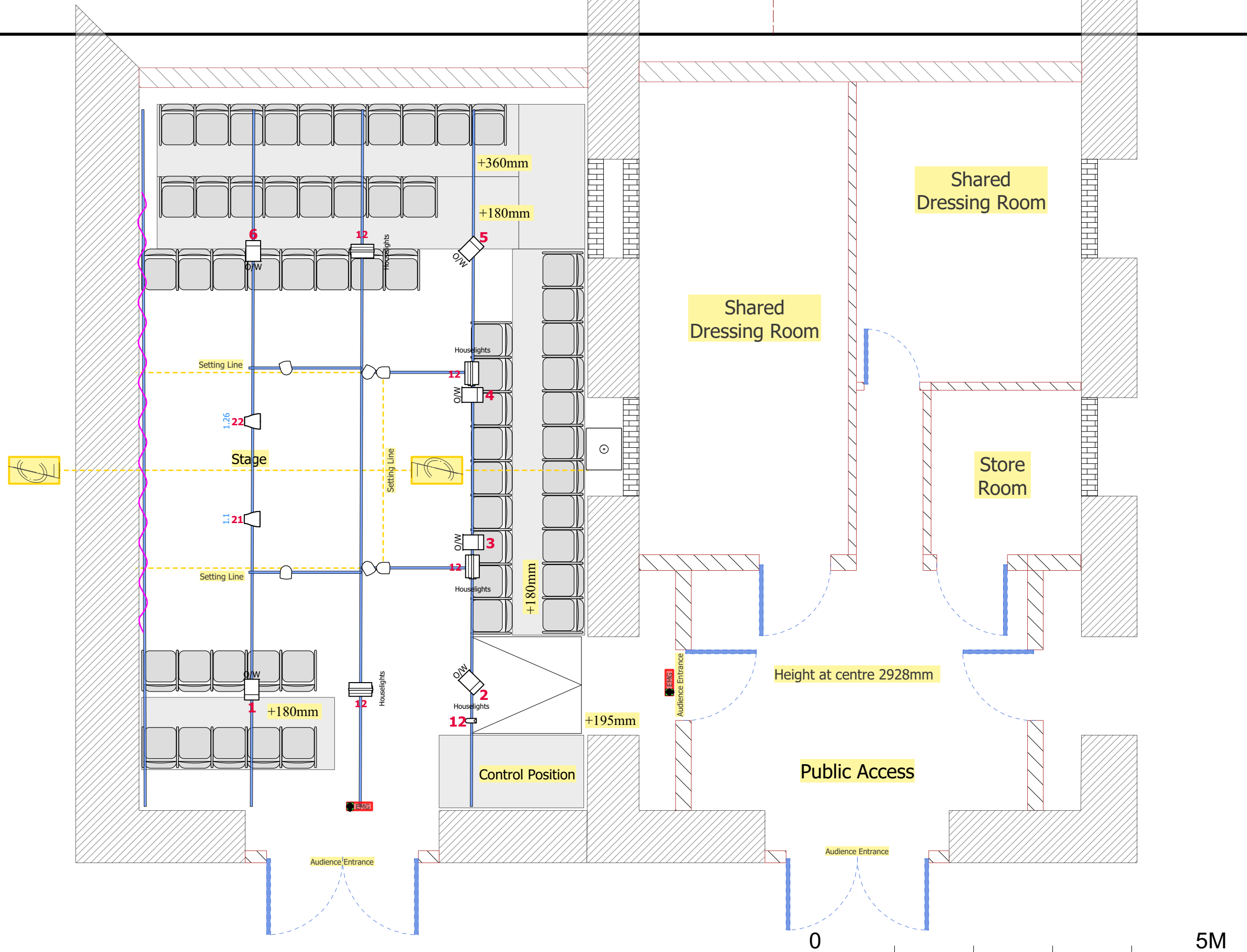
19/B2B/01 Bunker Two Venue Layout - Website View Scale: 1:50
