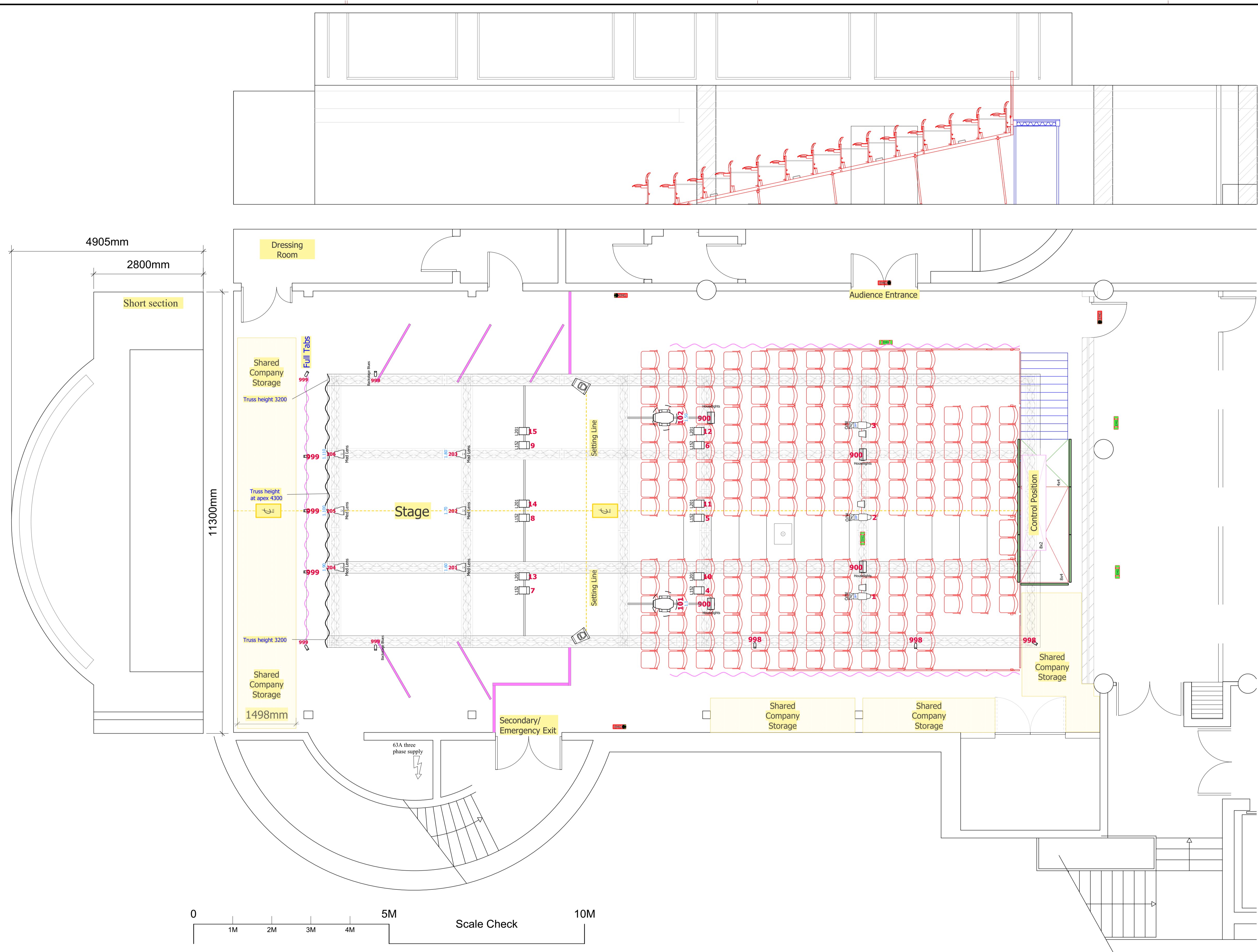
19/KD/01 Pleasance KingDome - Venue Layout - Website View Scale: 1:50
